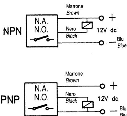
Schema collegamenti Connections diagram
