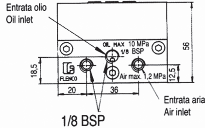
Overall dimensions
